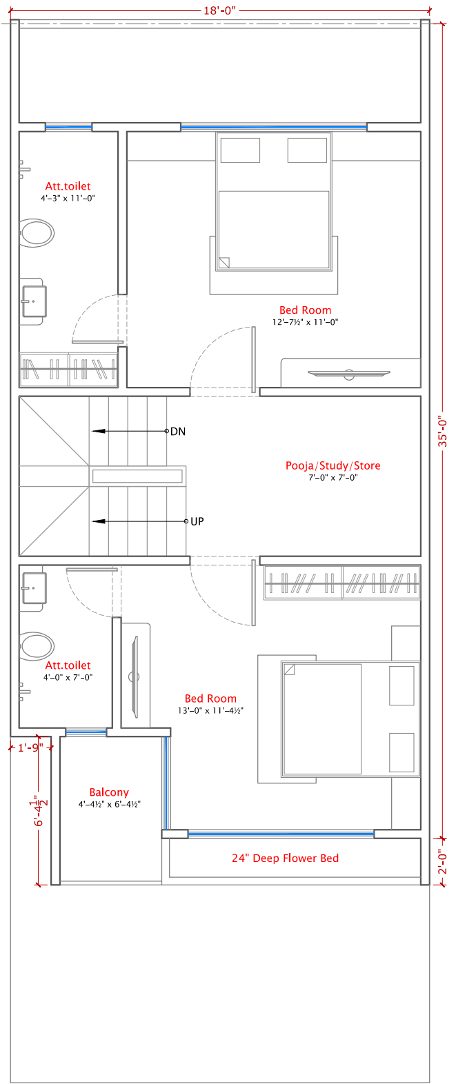
FIRST FLOOR
