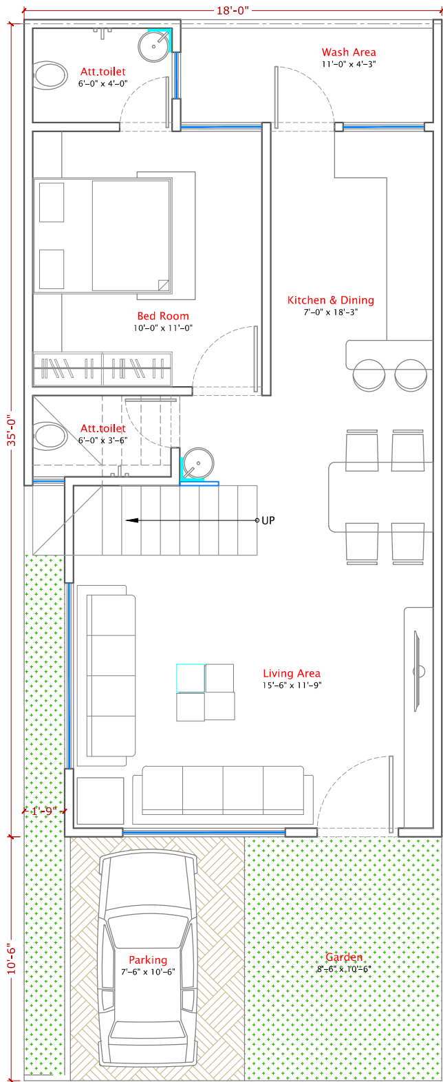
GROUND FLOOR
