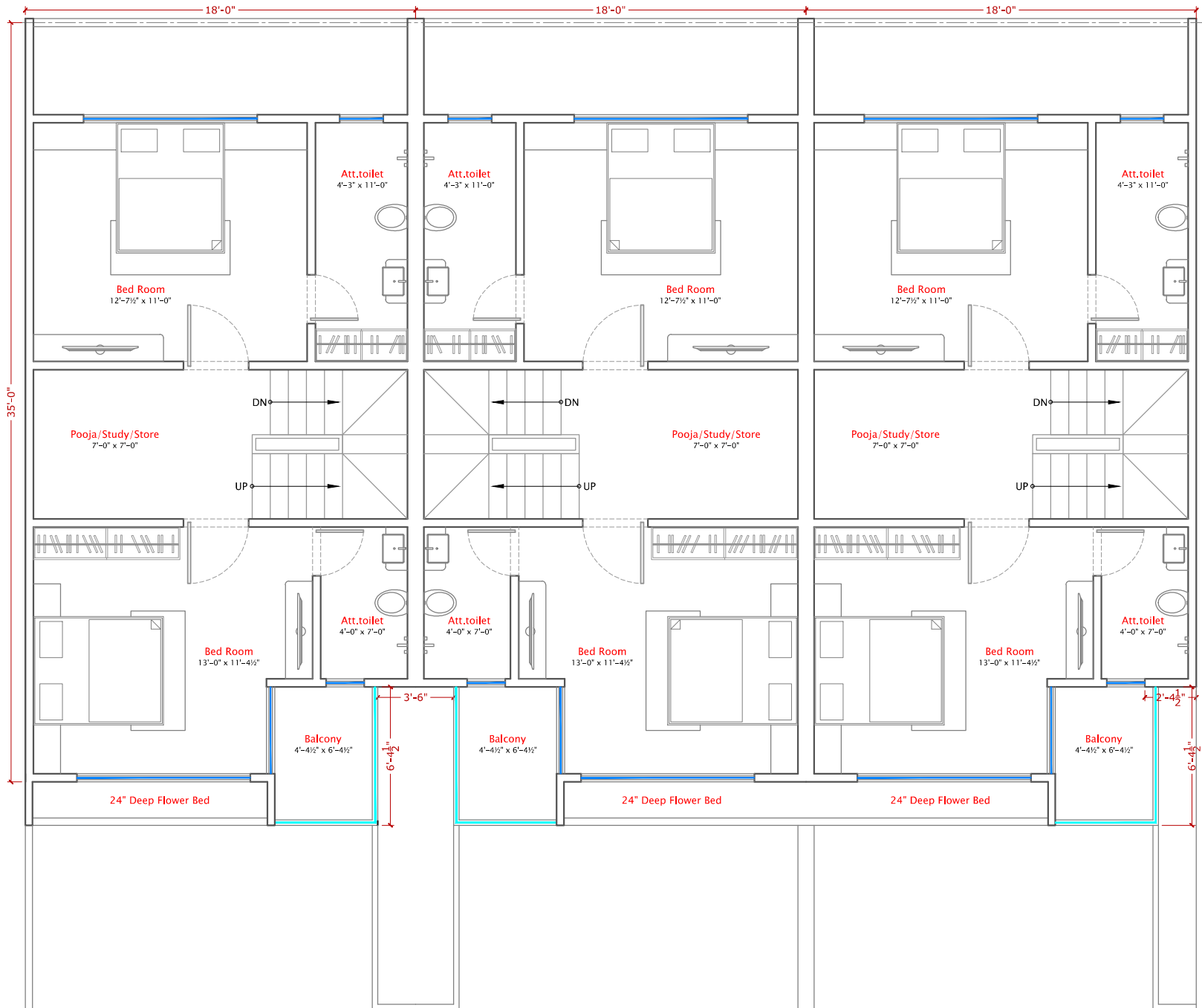
First Floor
