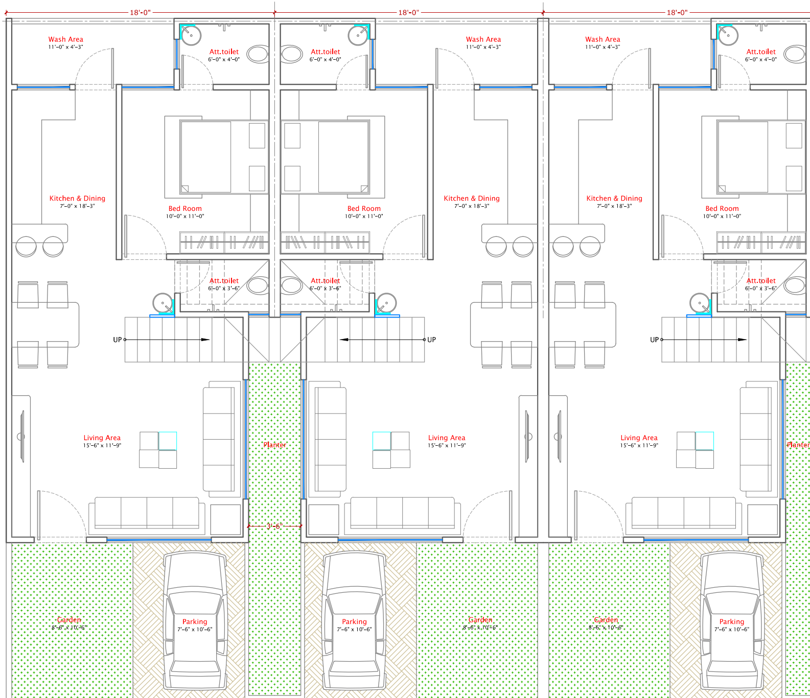
Ground Floor
